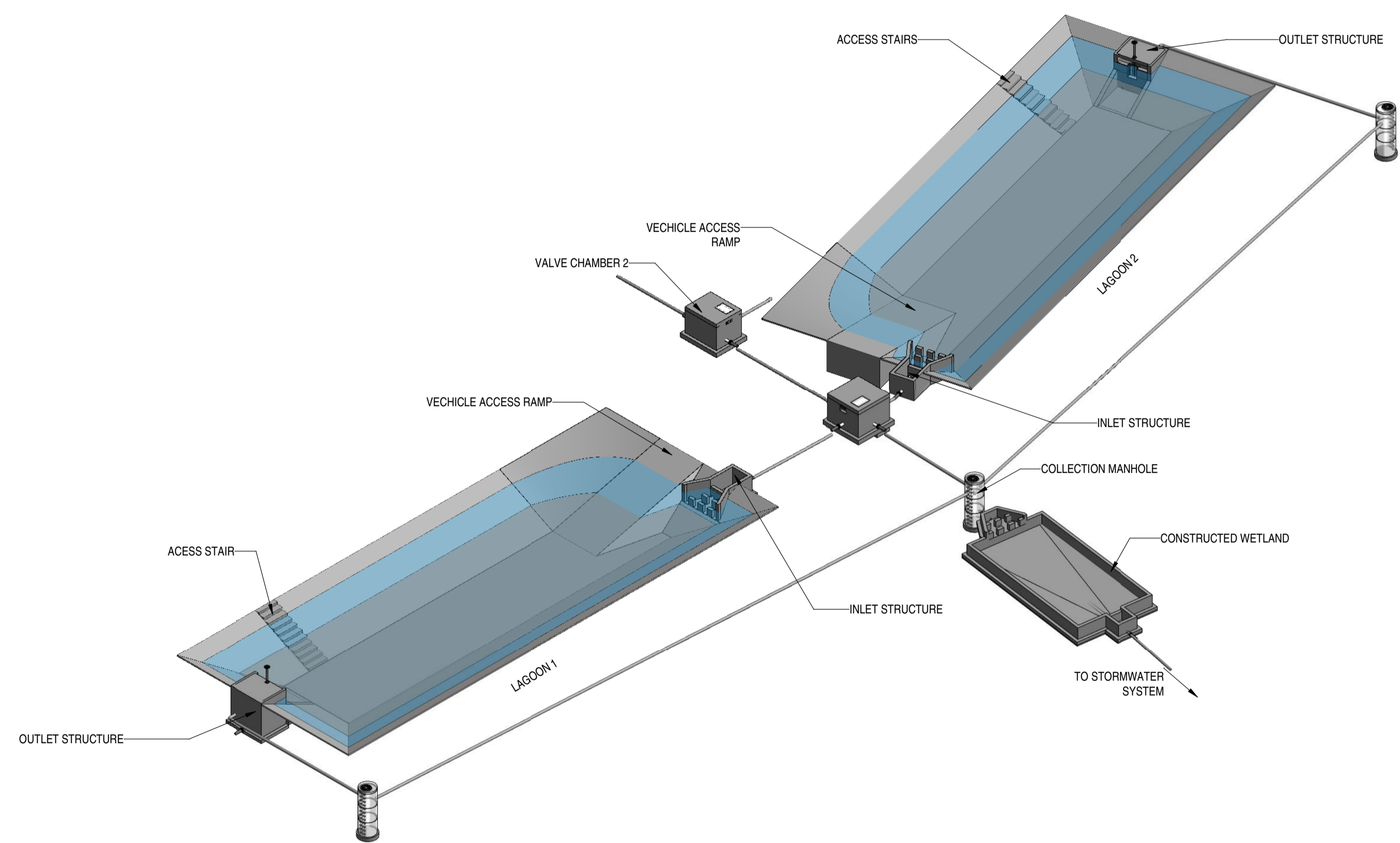
ISOMETRIC VIEW
