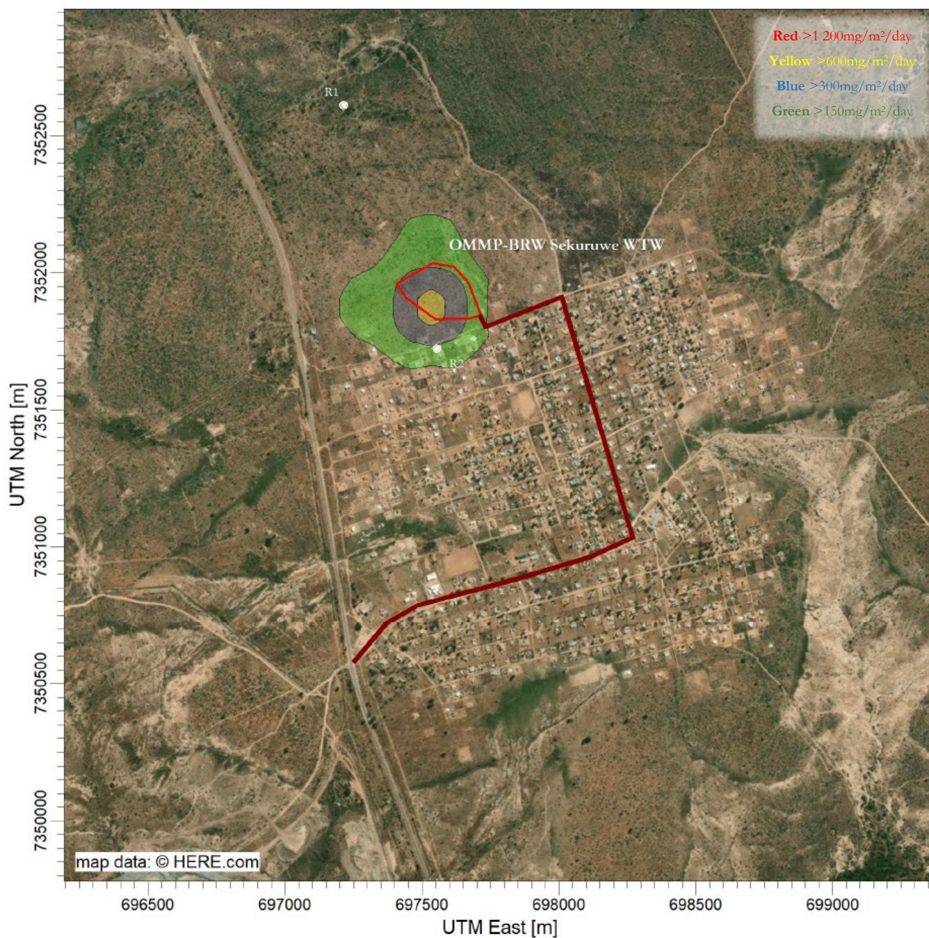
Figure 35: Daily Average Dust Deposition Rate – Construction/Rehabilitation (Non-residential Standard – 1\,200\text{mg}/\text{m}^2/\text{day} , Residential Standard – 600\text{mg}/\text{m}^2/\text{day} )
