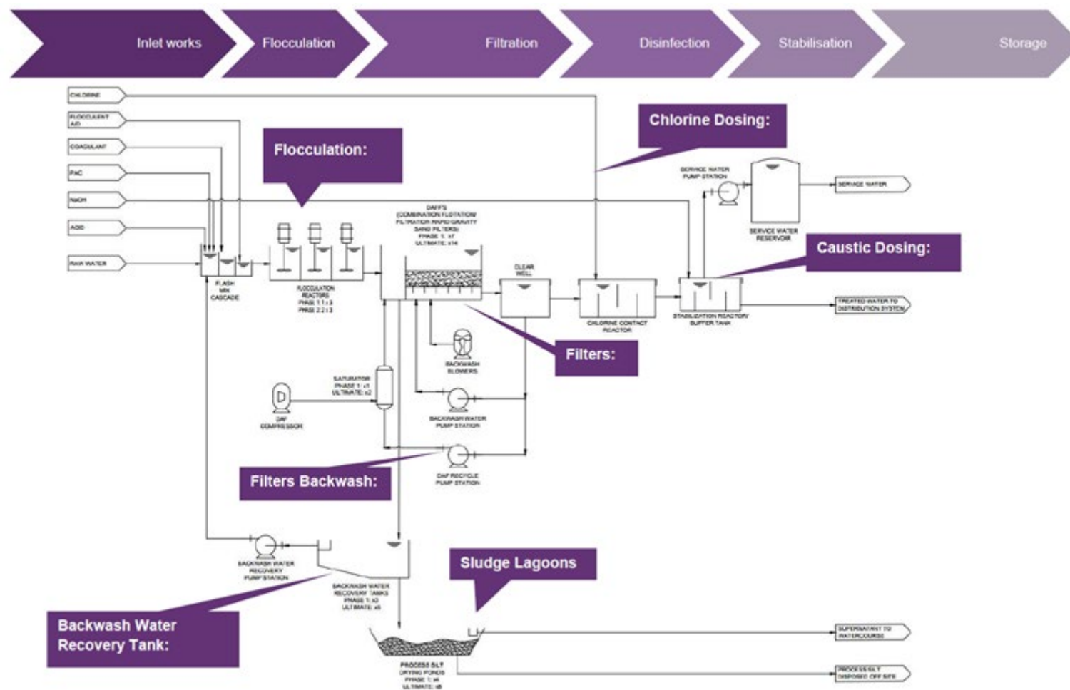
Figure 12: Sekuruwe WTW Process Flow Diagram
