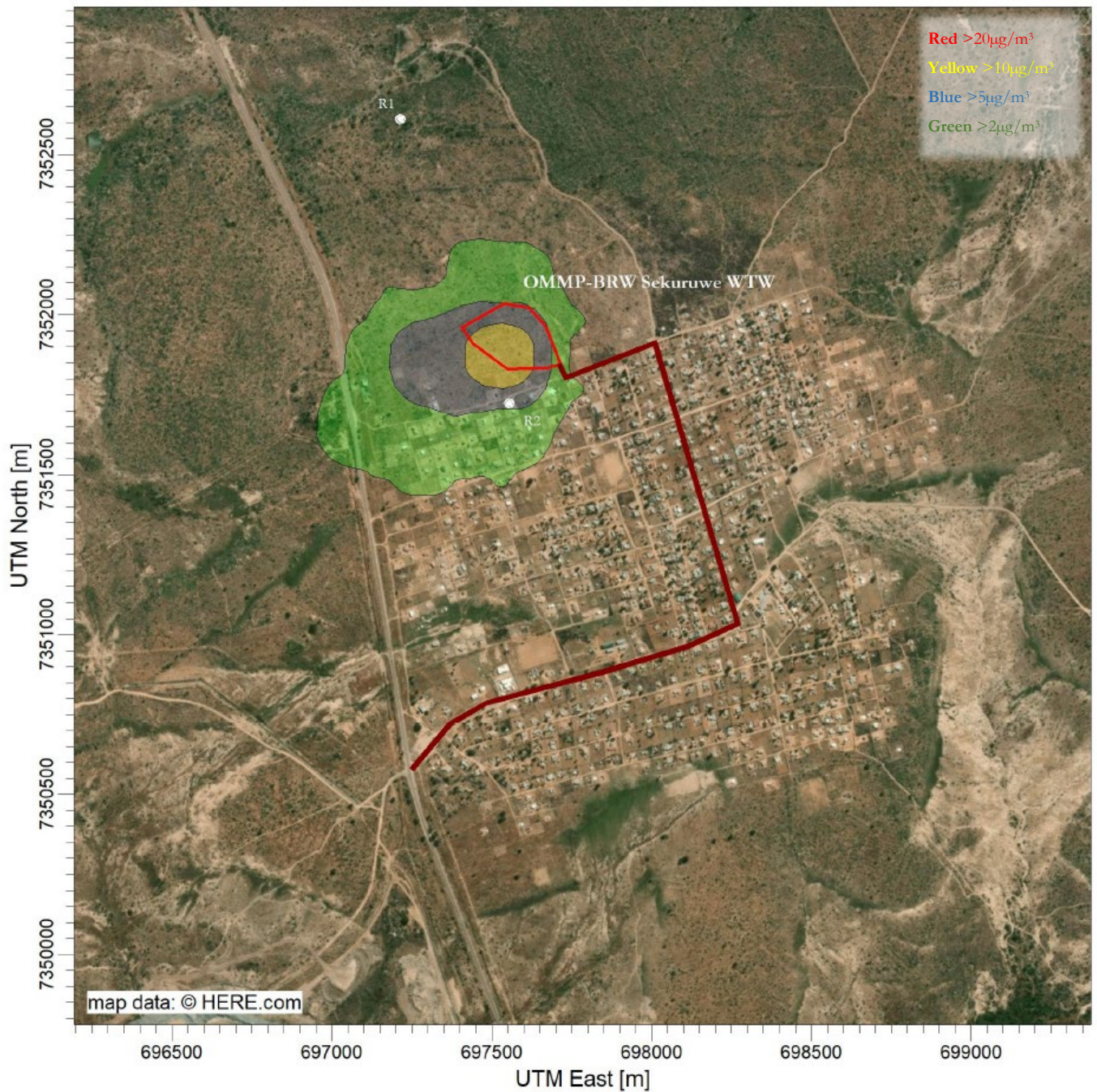
Figure 36: Annual Average Chlorine Concentration – Operations (US EPA RfC – 20\mu\text{g}/\text{m}^3 )
