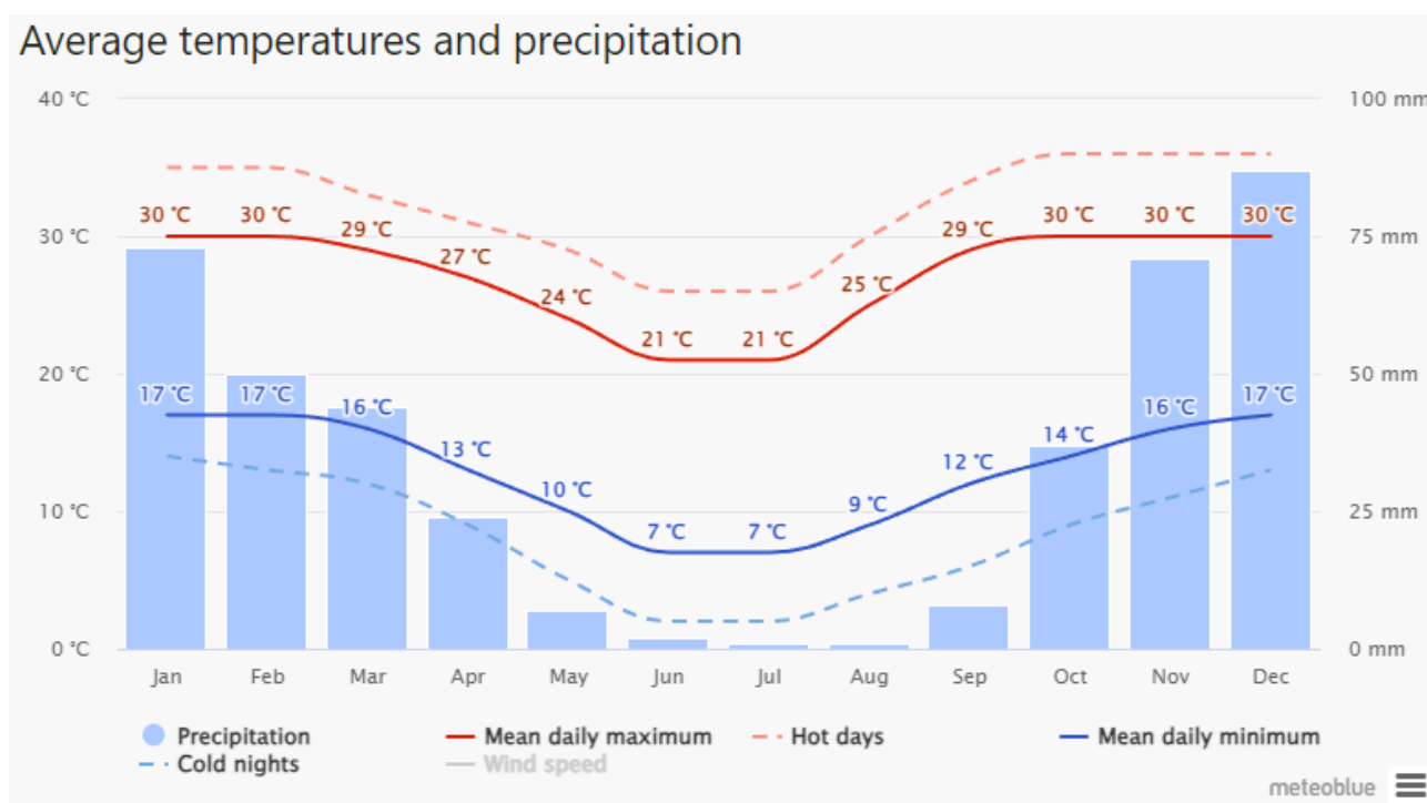
Figure 23: Mokopane Average Temperature and Precipitation for the Period 1992 – 2023
