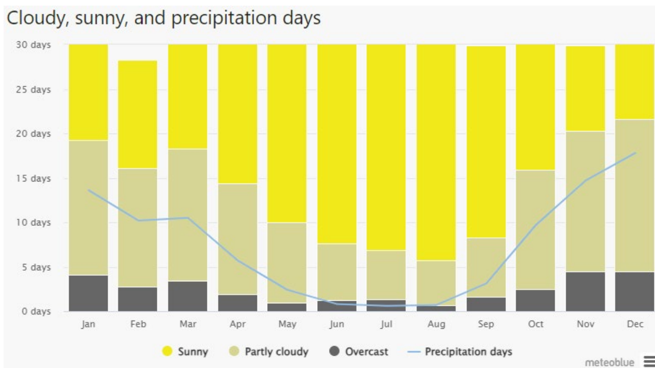
Figure 25: Mokopane Cloud Cover and Precipitation Days for the Period 1992 – 2022
