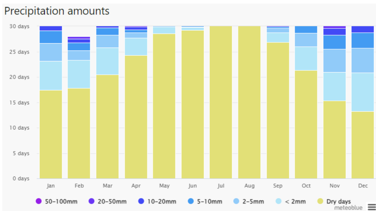
Figure 24: Mokopane Average Monthly Rainfall for the Period 1992 – 2022
