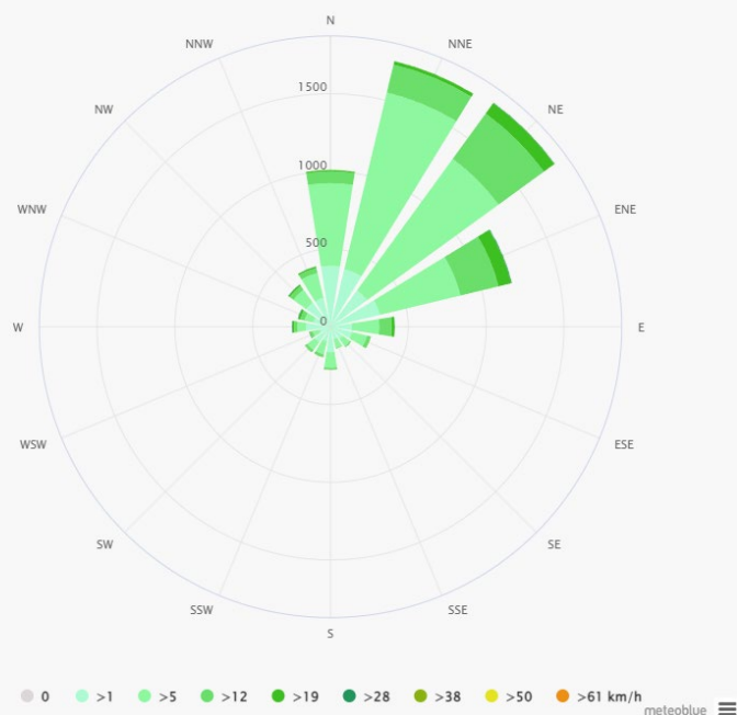
Figure 13: Mokopane Wind Rose for the Period 1992 – 2022
