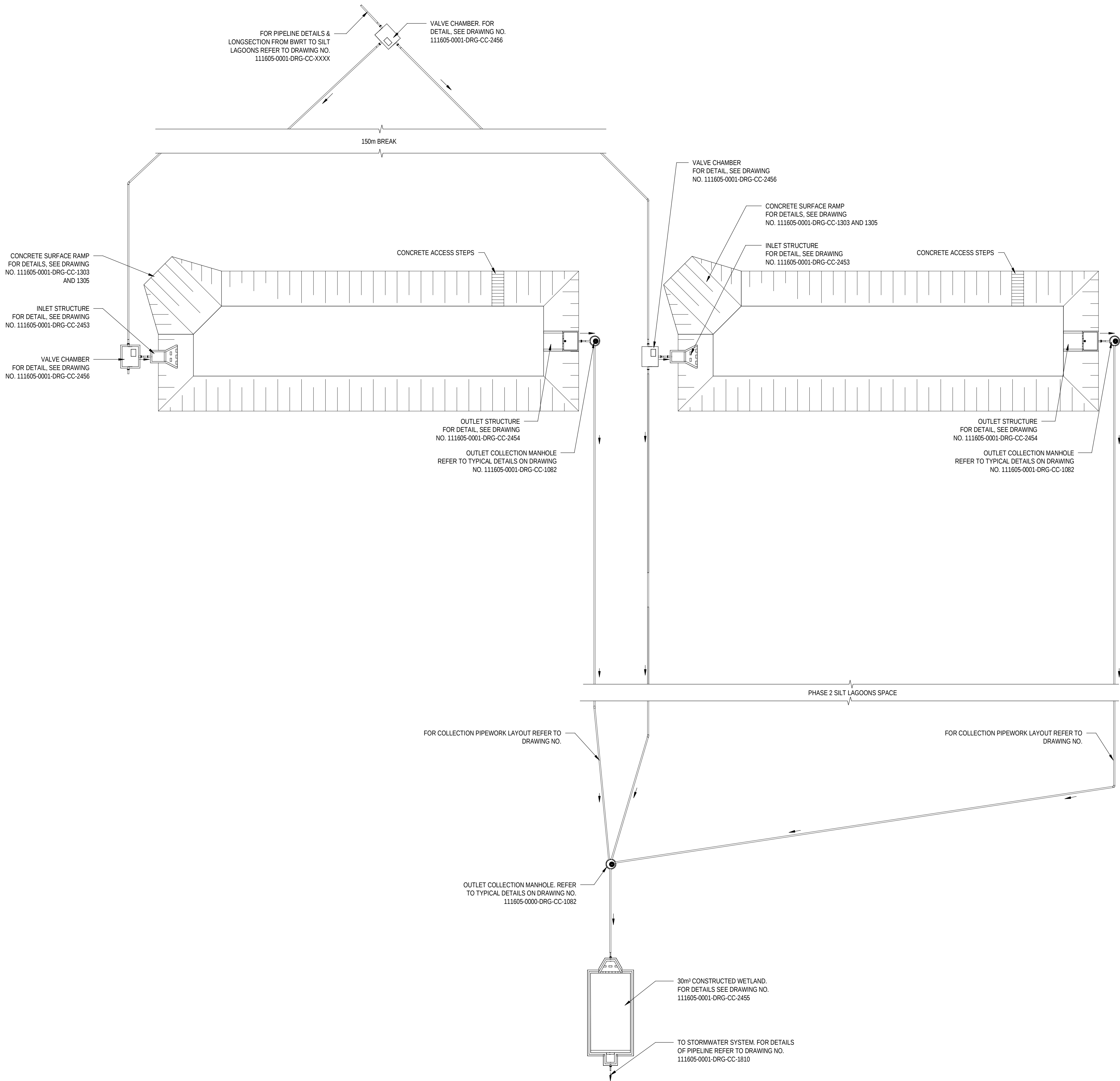
GENERAL ARRANGEMENT 1 : 250
