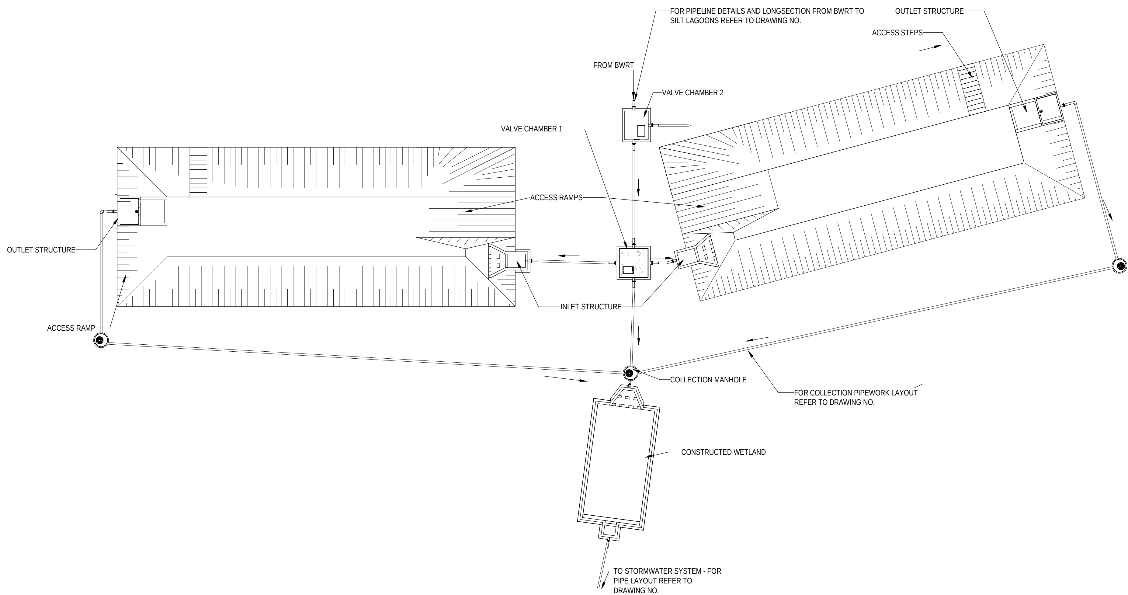
GENERAL ARRANGEMENT 1 1 : 200
