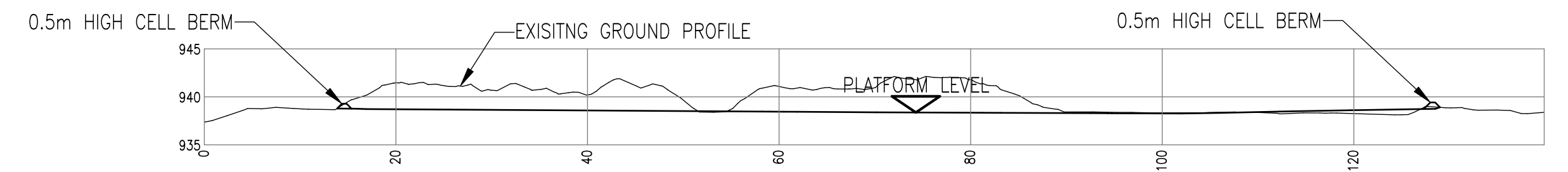
SECTION A SCALE 1:500
