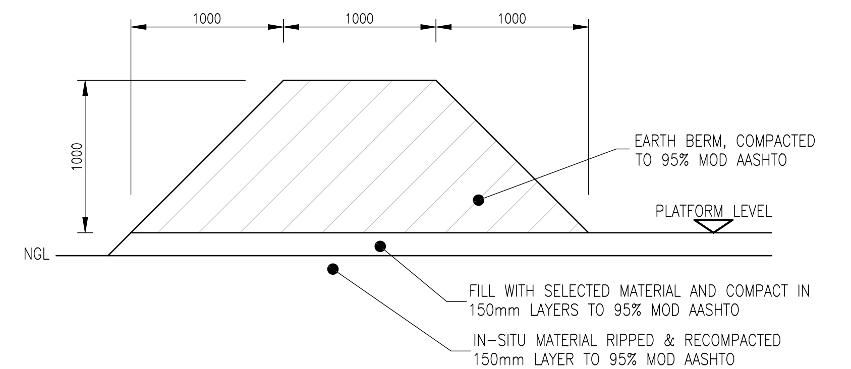
SECTION - CONTAINMENT BERM SCALE 1:25
