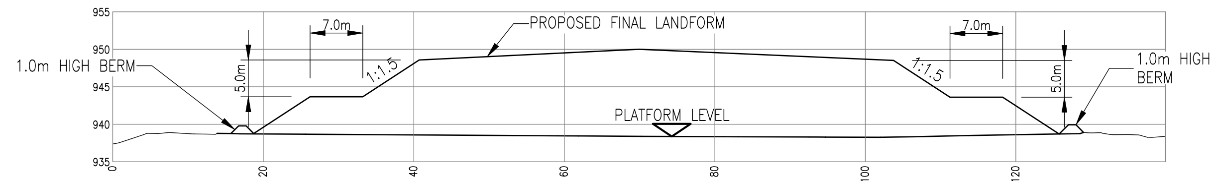
SECTION SCALE 1:500
