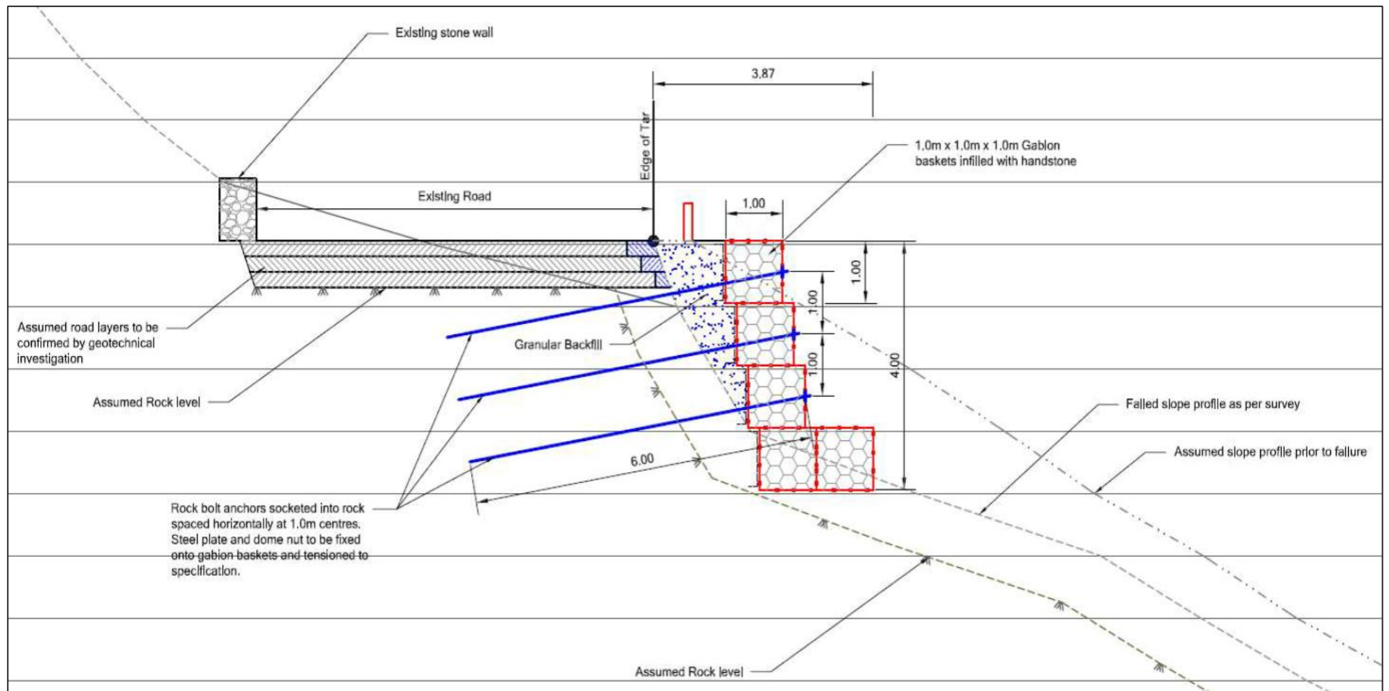
Figure 1: Anchored Gabion Wall
