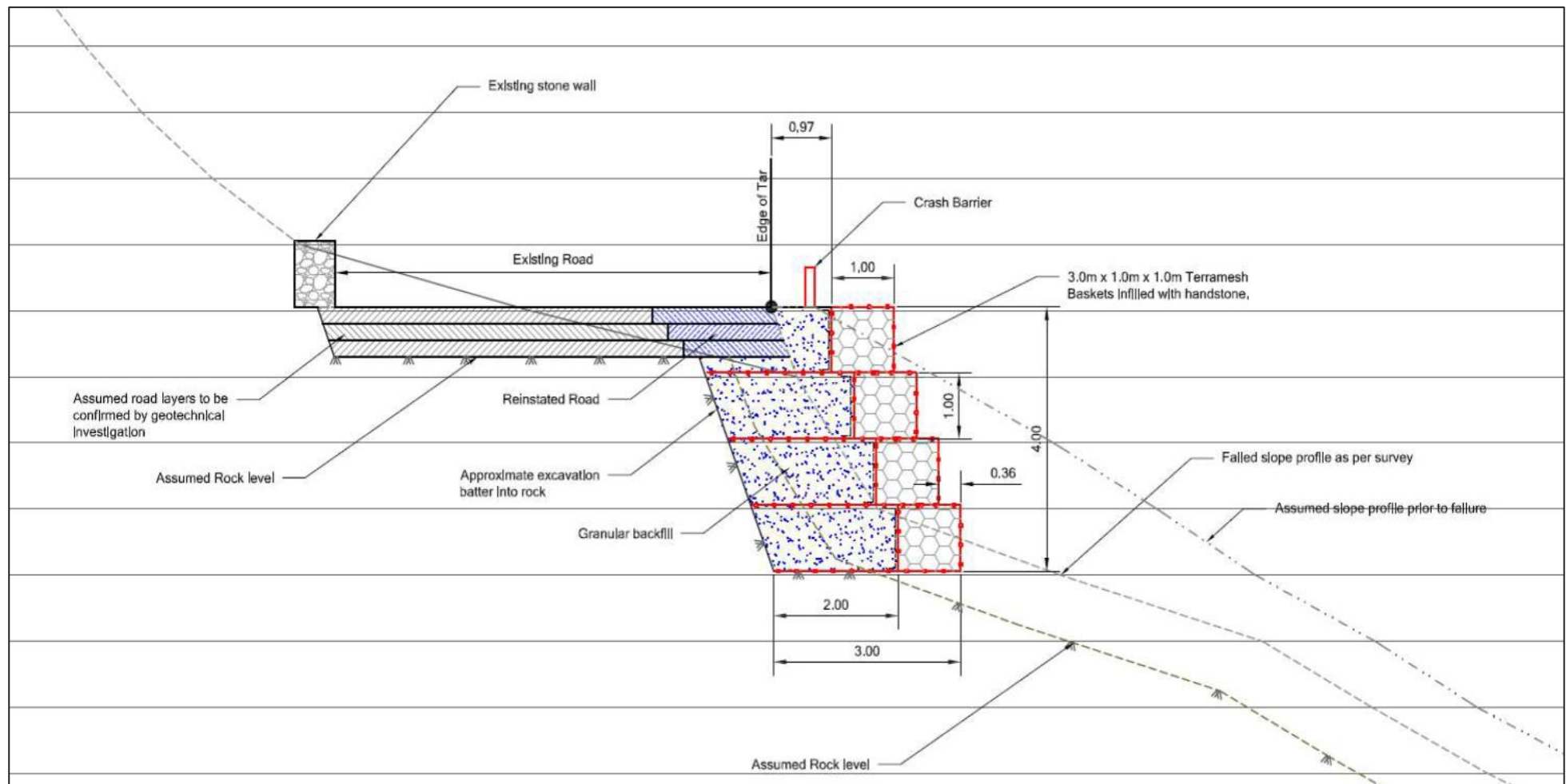
Figure 2: Terramesh Retaining Wall
